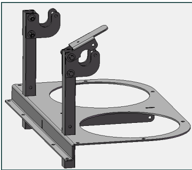
# BR-2-101 2 Bucket Carrier with Clamp Kit
