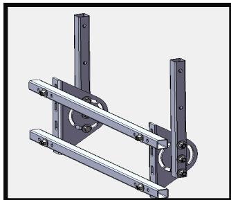
#UM-101-90 ATV Universal Mount
