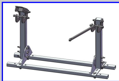
Universal Auger Mount
