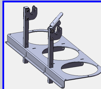
BR-3-101 3 Bucket Rack Holder
