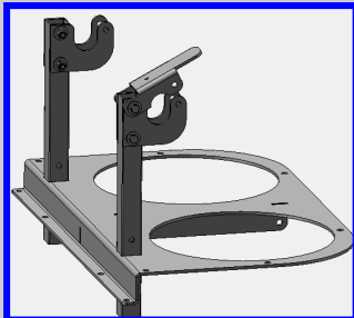
BR-2-101 2 Bucket Rack Holder
