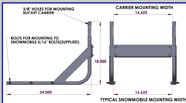
CK-1 Clamp Kit
